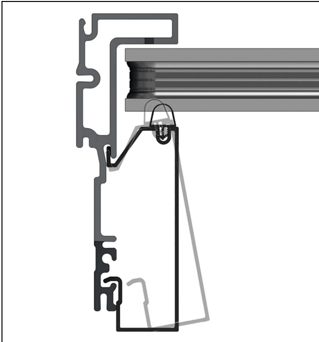
Figure 39 Rectangular covers
