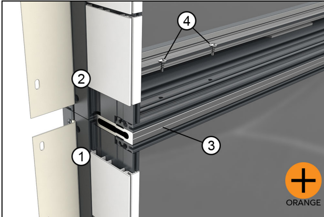
Figure 37 Horizontal mull (framing not shown for illustrative purpose)
