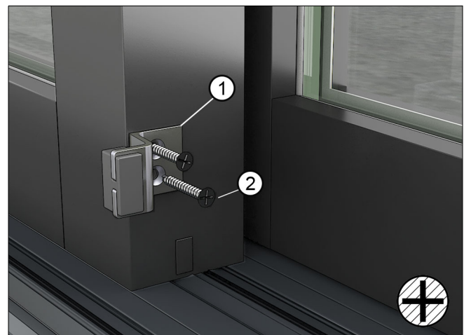
Figure 88 Bottom secondary panel bumper
