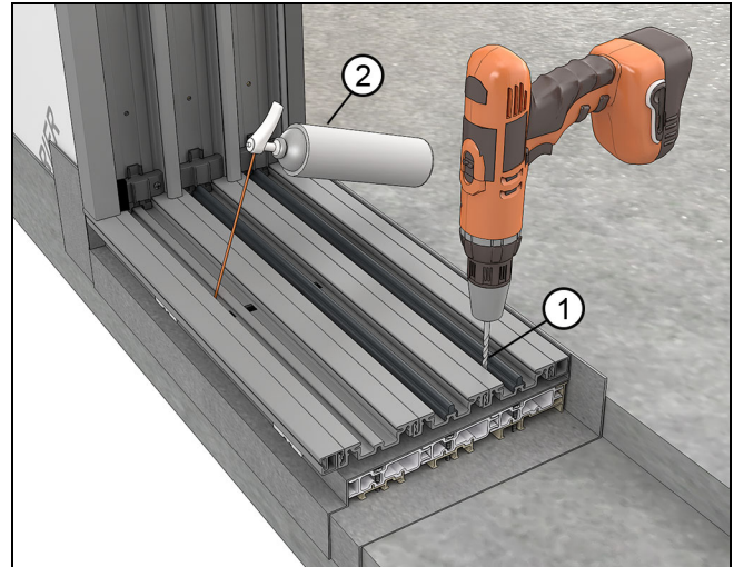
Figure 57 Drilling through HP stacked sill.
