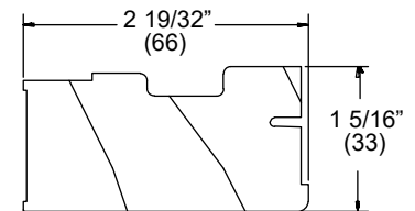
Astragal, W7717 Replace with the Astragal Assembly
