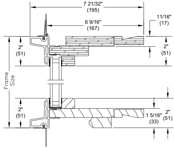
DOUBLE HUNG/DOOR - 6 9/16"
