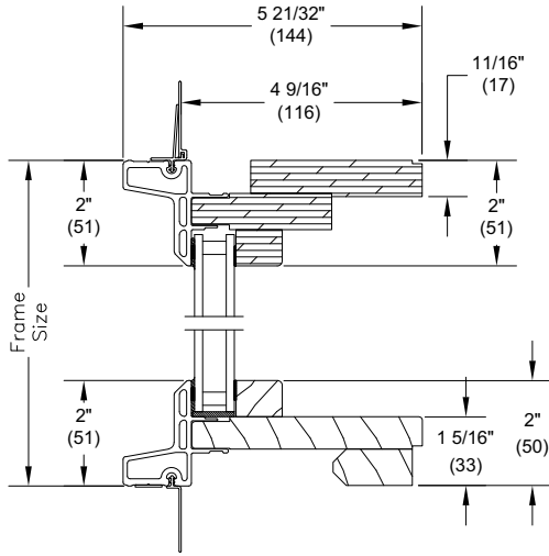
DOUBLE HUNG/DOOR - 4 9/16"
