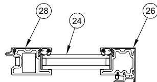
1 5/16" Bi-parting Panel
