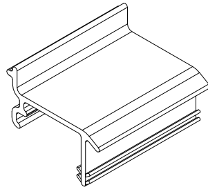
Vinyl Spacer, V2573
