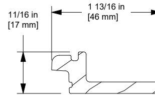
Removable Interior Jamb Cover, W13093
