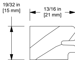
Jamb Liner, Picture, W12569
