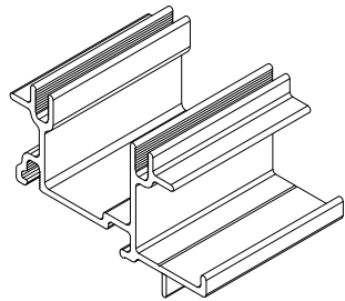
Mid Exterior Cover Base, V2432
