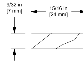
14 Degree Sill Liner, Operator, W12515
