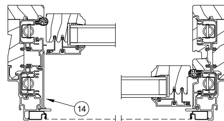
Single Hung Jamb Detail
