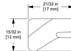
Head Jamb/Jamb Stop, W12407
