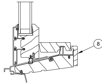
8 Degree Sill Vertical Detail
