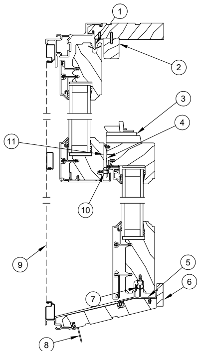
Head Jamb and 14 Degree Sill Vertical Detail
