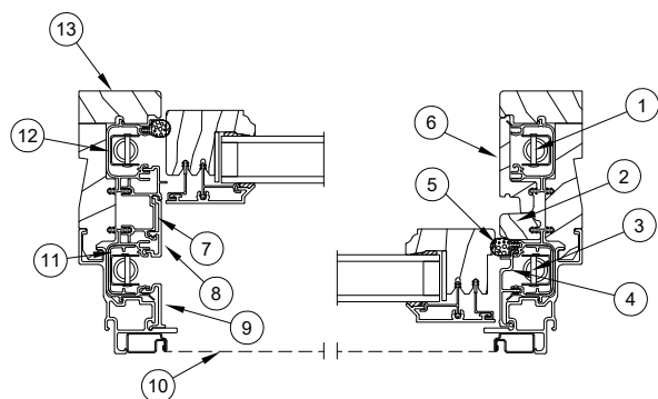
Double Hung Jamb Detail
