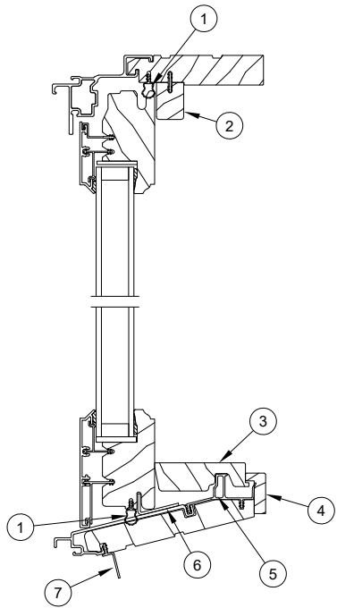
Head Jamb and 14 Degree Sill Vertical Detail
