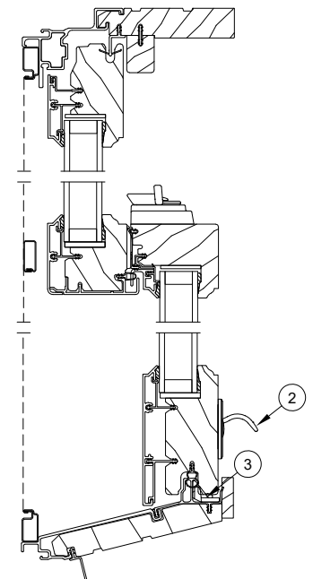
Head Jamb and Sill Lift Lock (Single Hung Only)
