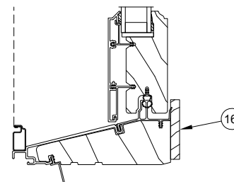
Flat Degree Sill
