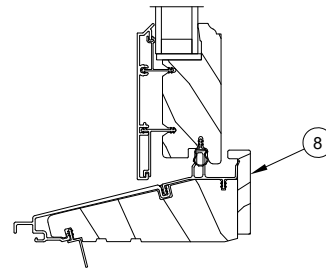
0 Degree Flat Sill Vertical Detail
