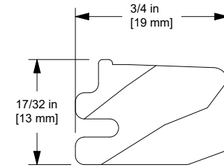
Fixed Interior Jamb Cover, W13094
