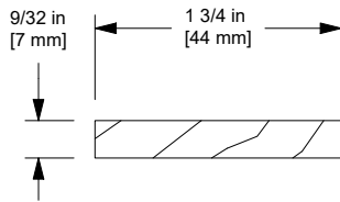
0 Degree Sill Liner, Operator, W12595
