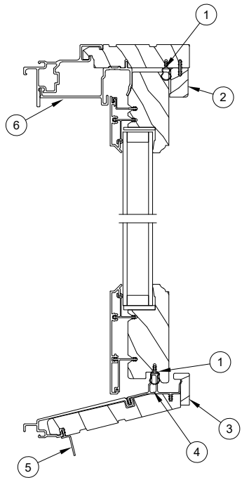
Head Jamb and 14 Degree Sill Vertical Detail
