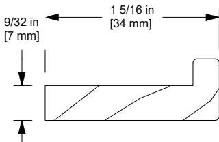
8 Degree Sill Liner, Picture/Transom, W11825
