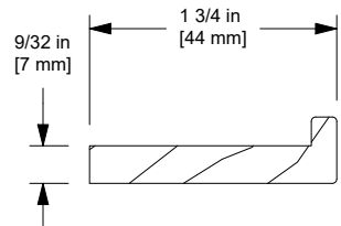
0 Degree Sill Liner, Picture/Transom, W12597
