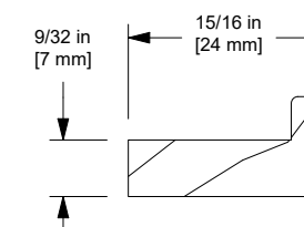
14 Degree Sill Liner, Picture/Transom, W12566
