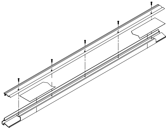
Pull Bar and Backer with Fin and screws
