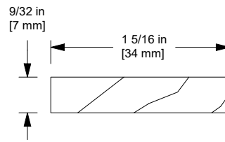
8 Degree Sill Liner, Operator, W11576
