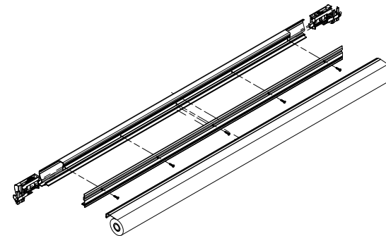
Screen Cartridge Assembly, Partial
