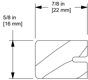
Parting Stop, W11578
