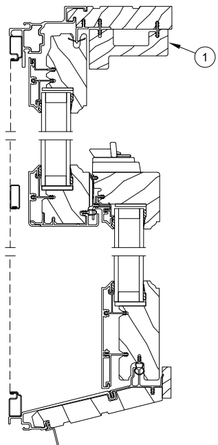
Head Jamb and Sill With Lock Status Sensor
