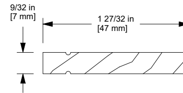
Sill Liner, W2146
