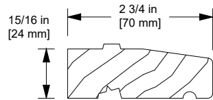
Subsill, W10333
