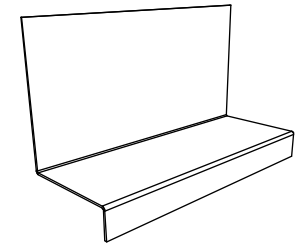
Drip Cap (Aluminum Flashing), A101
