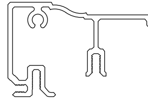
Clad Brick Mould Casing A232
