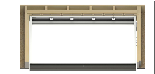
Figure 2 Block Placement for Head Jamb.
