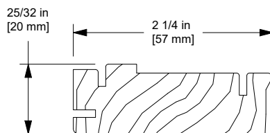
W8986 Head Jamb/Jamb Stop 2 1/4" Door No longer available Used prior to 3/30/2009
