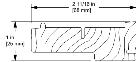
W2136 Head Jamb/Jamb Parting Stop Operator and In-Sash Transom
