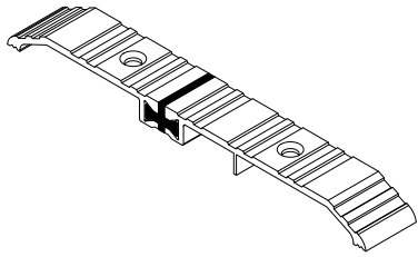
1/2" Sill (Profile#253) Standard Sill Pemko Model 253X4AFG (Anodized Aluminum) Options: 253X4DFG (Dark Bronze)
