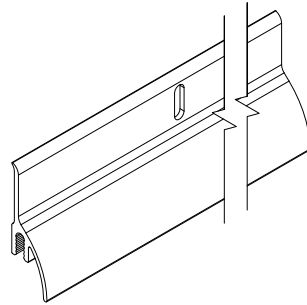
A2408 Panel Drip
