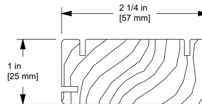
W12095 Head Jamb Stop 2 1/4" Door (use with Von Duprin 5547 Hardware Prep)
