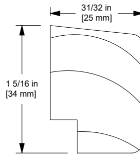
W12031, Sill Nosing Direct Glaze Rectangle (Total R.O. Continuous Casing) Pre-2011
