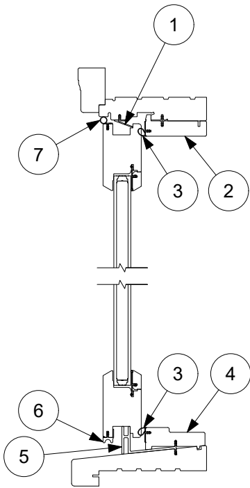
Head Jamb and Sill
