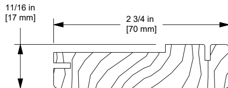
W9475 Head Jamb/Jamb Parting Stop Stationary
