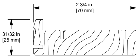
W6000 Head Jamb/Jamb Parting Stop Operator and In-Sash Transom
