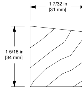
W12059 Sill Nosing
