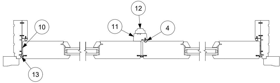
Stationary Jamb
