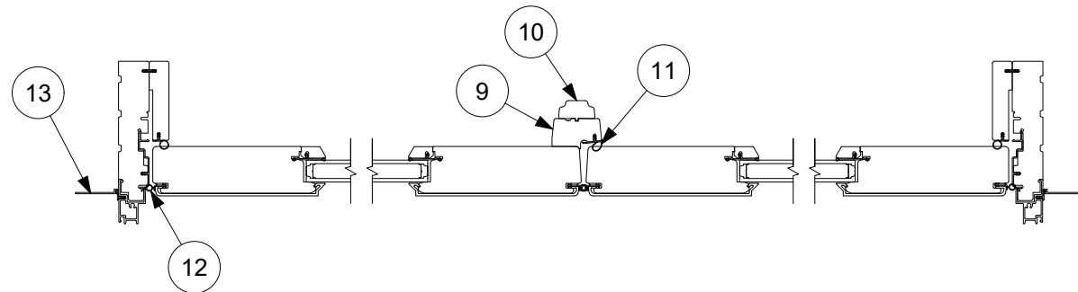
Stationary Jamb
