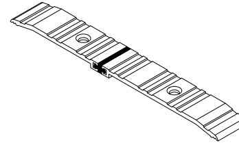
1/4" Sill (Profile#273) Thermal Barrier Threshold Pemko models: 273X4AFG and 273X4DFG
