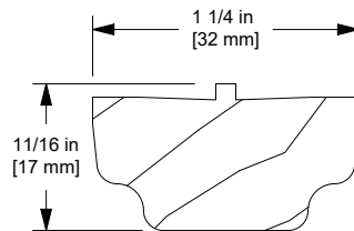
W7554 Mull Casing Cover
