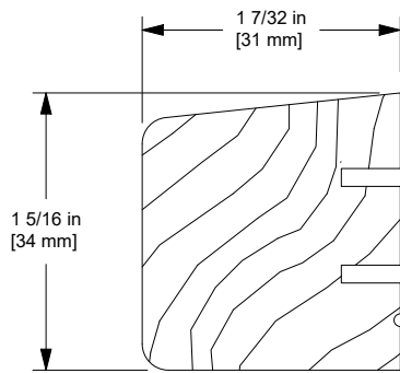
W8653, Sill Nosing Used prior to 6/24/2013
