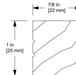
W14258 Glazing Bead, IG Direct Glaze Rectangle
