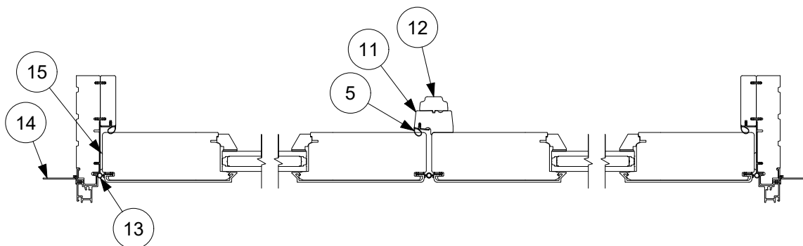
Stationary Jamb
