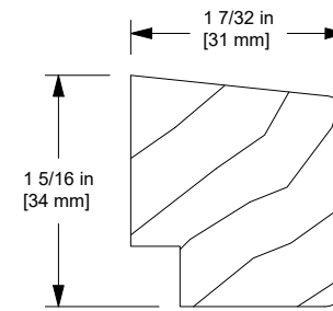
W12032, Sill Nosing Direct Glaze Rectangle Pre-2011 - Split Casing
