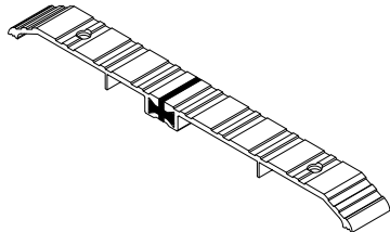
1/2" Sill Pemko Models: 254X5AFG and 254X5DFG
