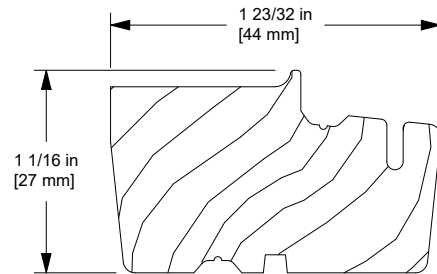
W1455 Mull Casing Base
