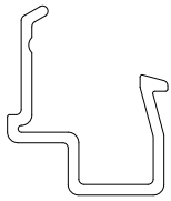
Jamb Adapter, A1958
